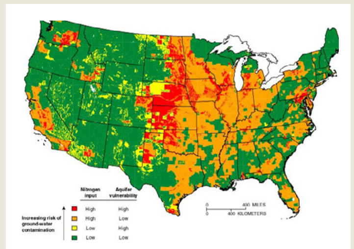
FIGURE 5: Risk of nitrate groundwater pollution. From USGS Circular 1225, The Quality of Our Nation's Waters .
